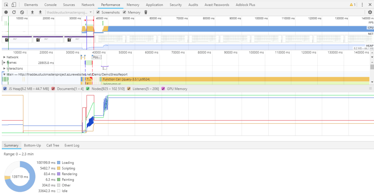
Figure 2: Performance Testing - Stress Testing on Azure Hosted Project Site
